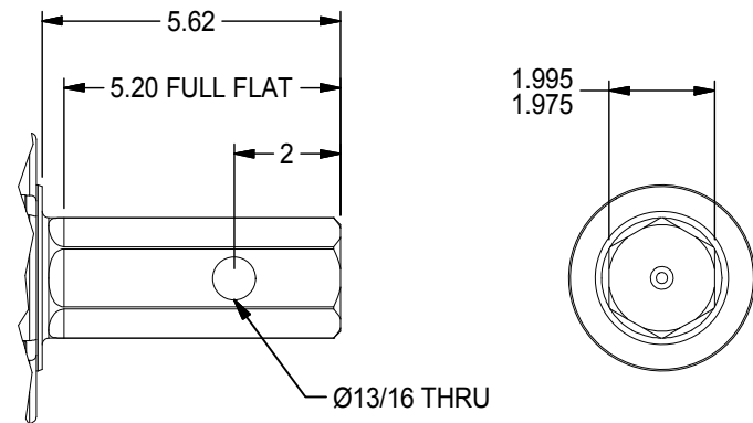
H2 Output Shaft 2" Hex
