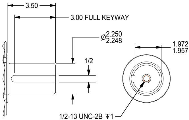
D3 Output Shaft \phi 2 \frac{1}{4} x 1/2 Keyway
