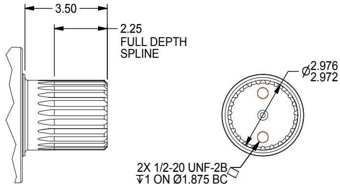
D1 Output Shaft 23T 8/16 DP Spline
